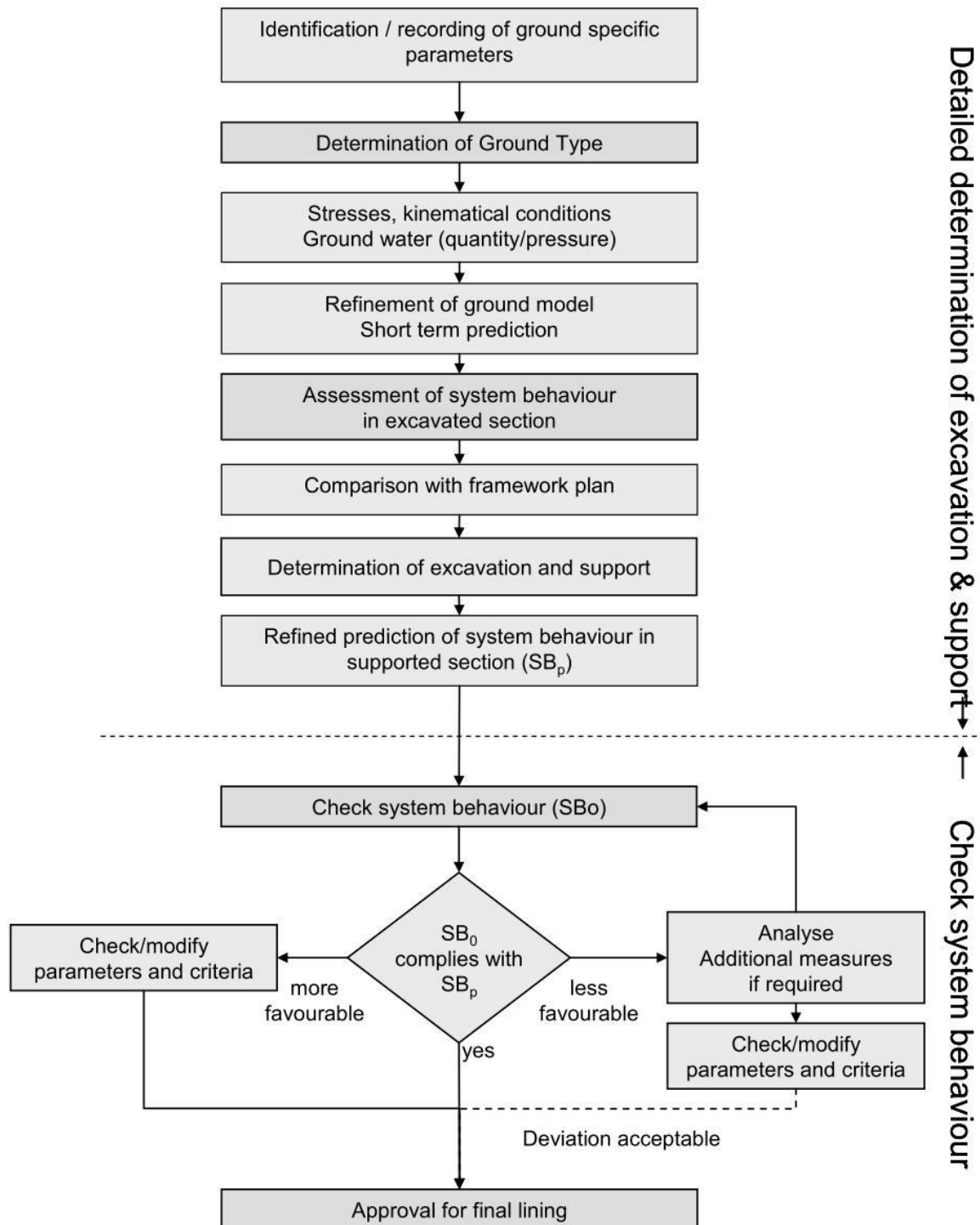
Figure 1: Basic procedure of determination of construction measures and check of system behaviour during construction ( SB_p = predicted system behaviour, SB_0 = observed system behaviour) from Austrian “Guideline for the
